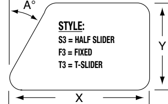
T-SLIDER
