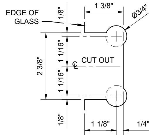
GLASS FABRICATION TEMPLATE
