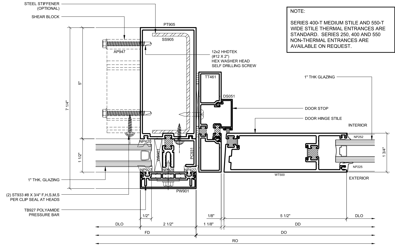
SECTION DETAIL @ DOOR JAMB 30
