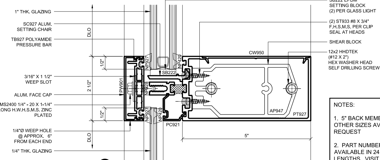
INT. HORIZ. SECTION 14 DOUBLE / SINGLE GLAZED 5\"/>
