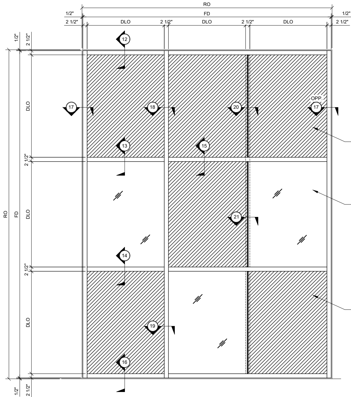
TYPICAL CURTAIN WALL ELEVATION
