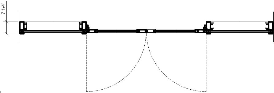
TYP. PLAN: THERMAL ENTRANCE WITH SUB-FRAME 1" THICK DOUBLE GLAZED 5" BACK MEMBER
