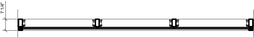
TYPICAL CURTAIN WALL PLAN
