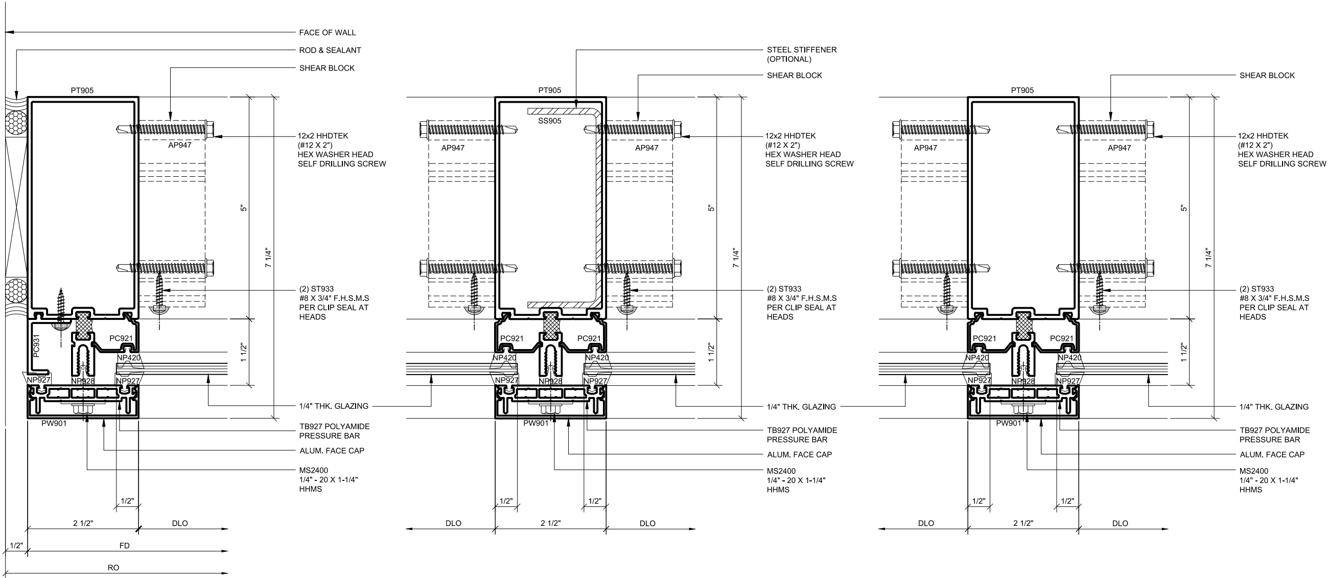
JAMB PLAN 17 SINGLE GLAZED 5" BACK MEMBER TRANSITION DETAIL 1'-0"=1'-0"
