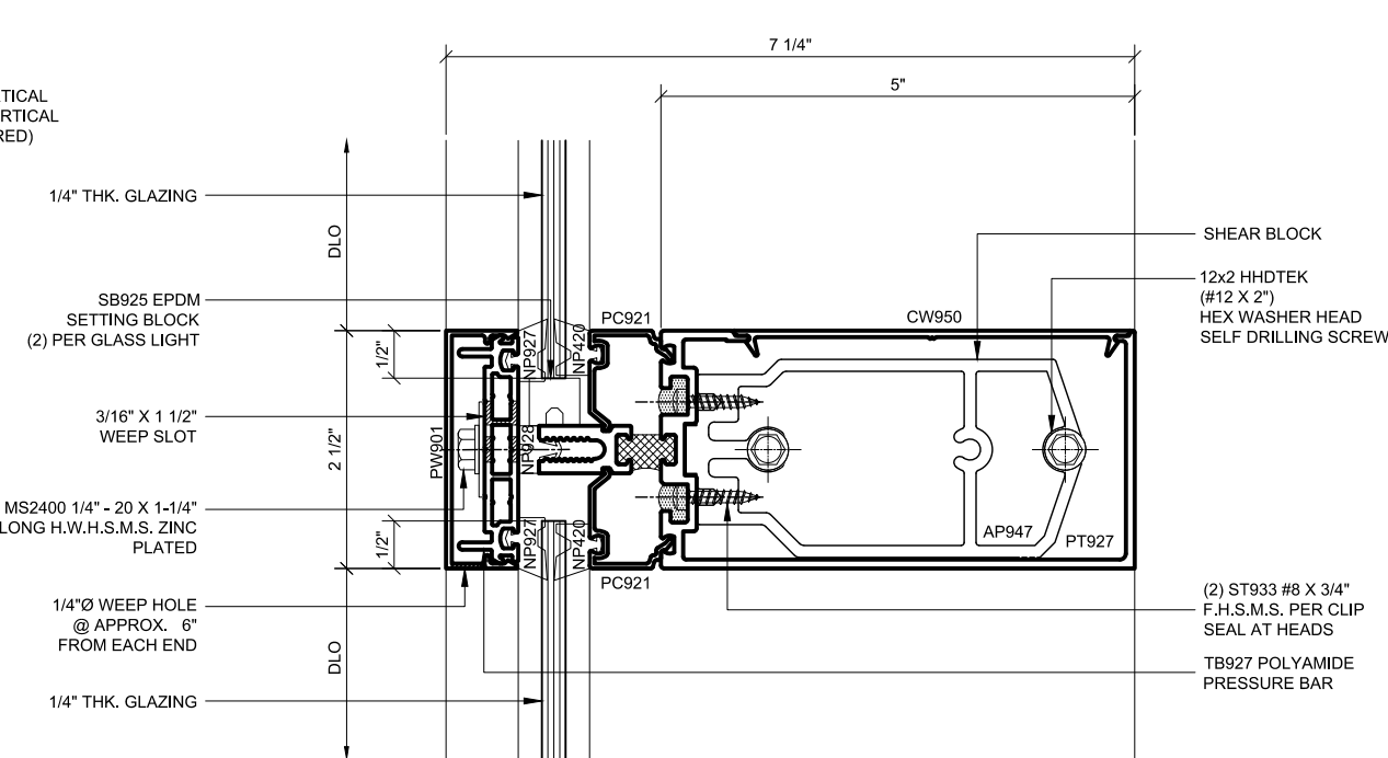
INT. HORIZ. SECTION 15 SINGLE GLAZED 5\"/>
