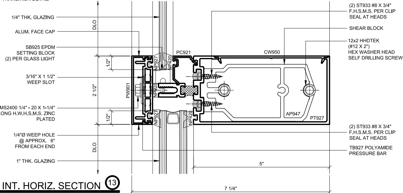
HEAD SECTION 12 SINGLE GLAZED 5\"/>
