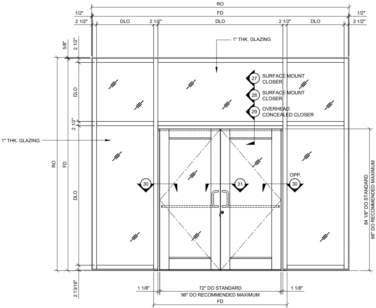
TYP. ELEVATION: THERMAL ENTRANCE WITH SUB-FRAME 1" THICK DOUBLE GLAZED 5" BACK MEMBER
