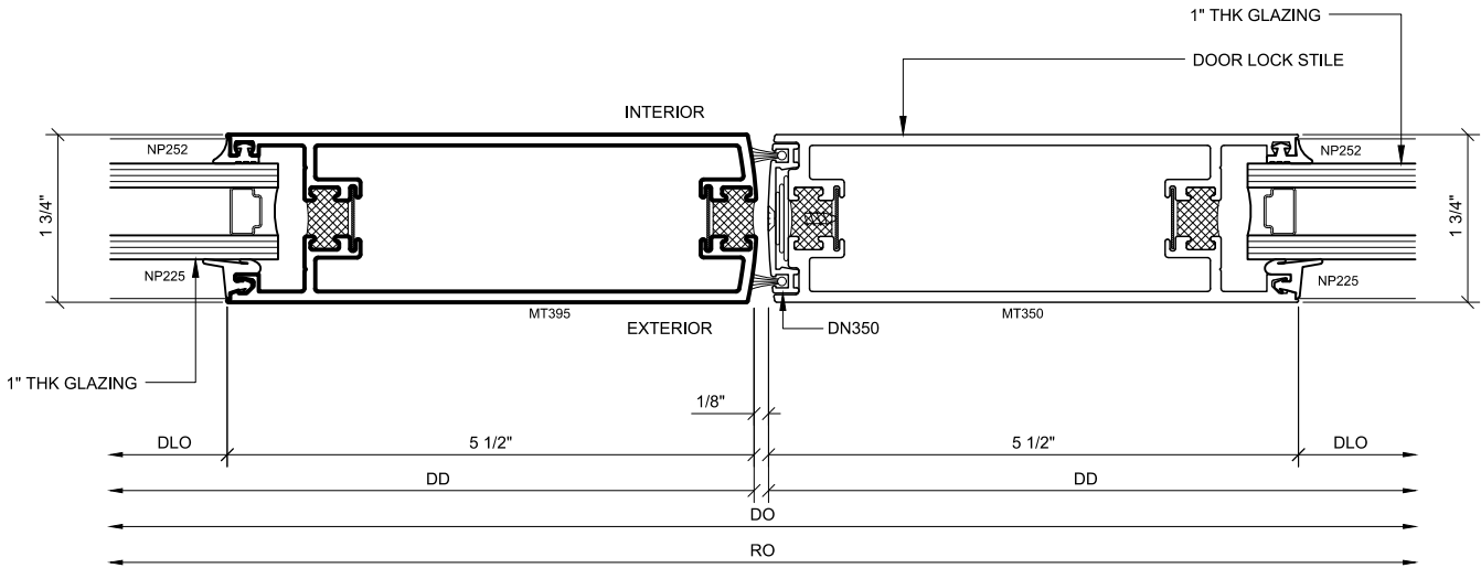
SECTION DETAIL @ MEETING STILES 31
