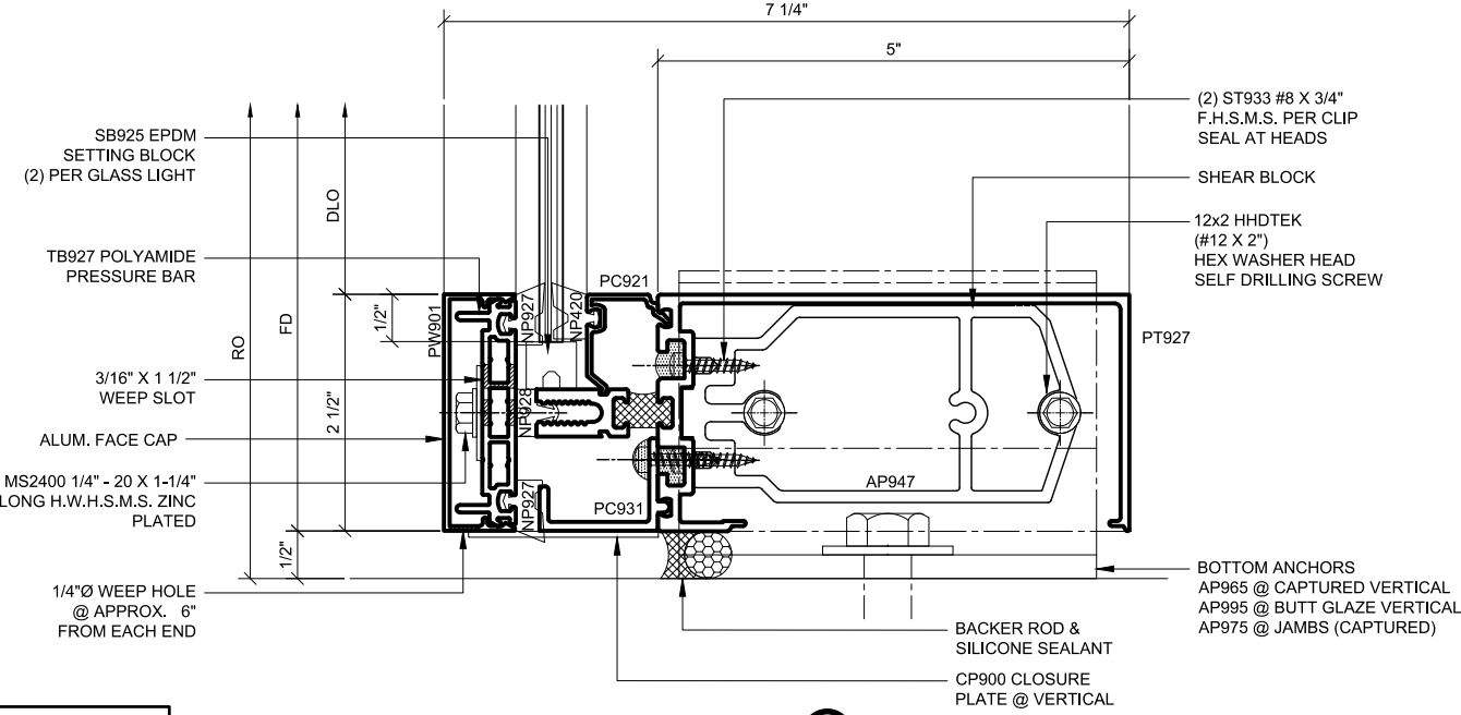
SILL SECTION 16 SINGLE GLAZED 5\"/>
