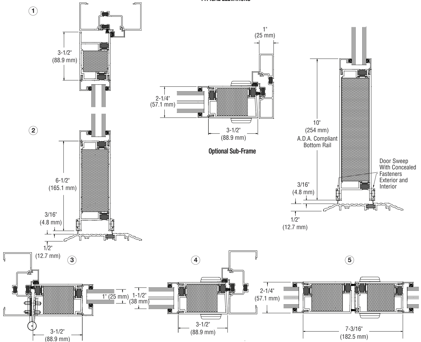
TYPICAL ELEVATIONS
