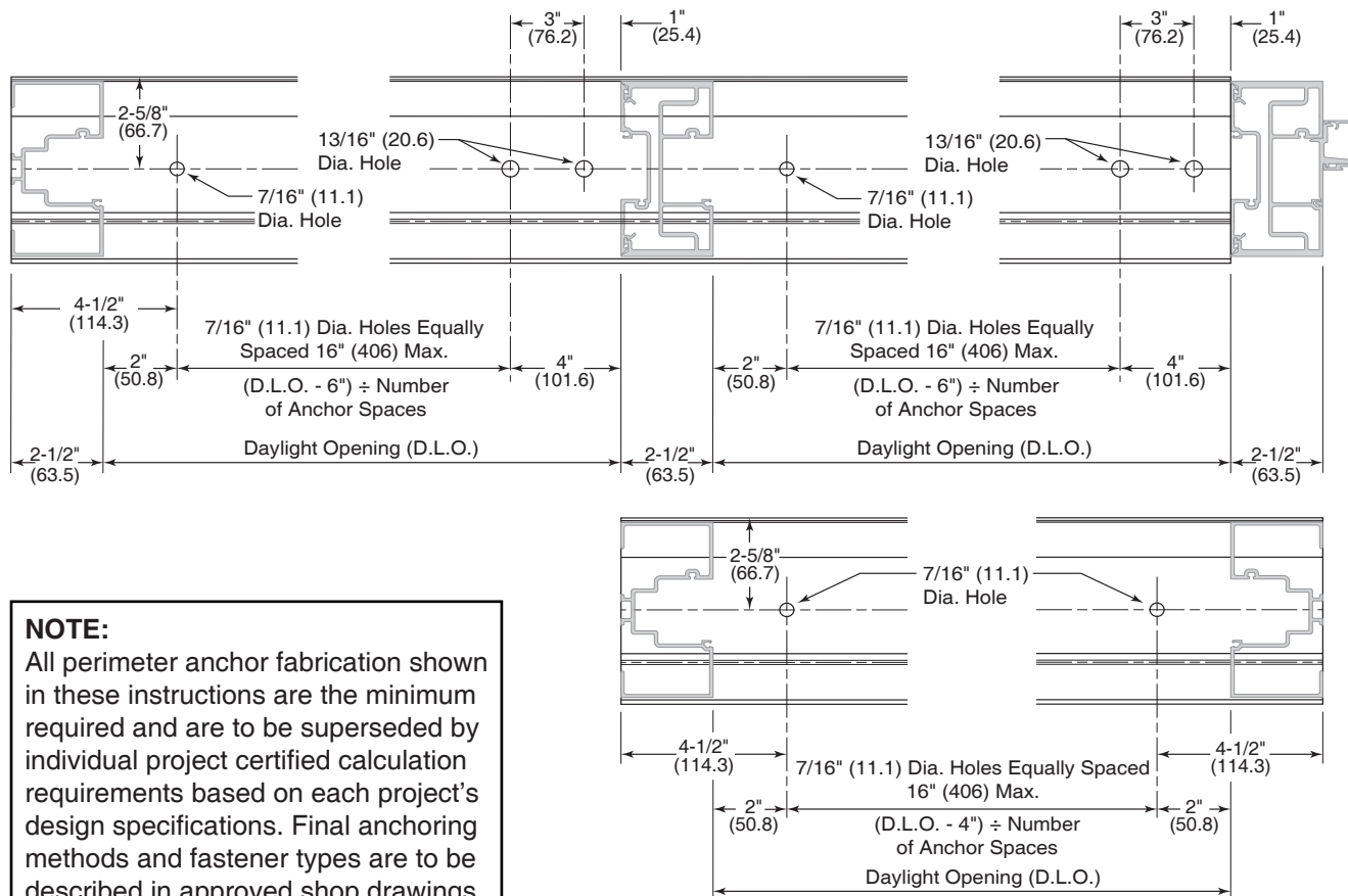
DETAIL D
