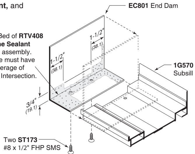
DETAIL I
