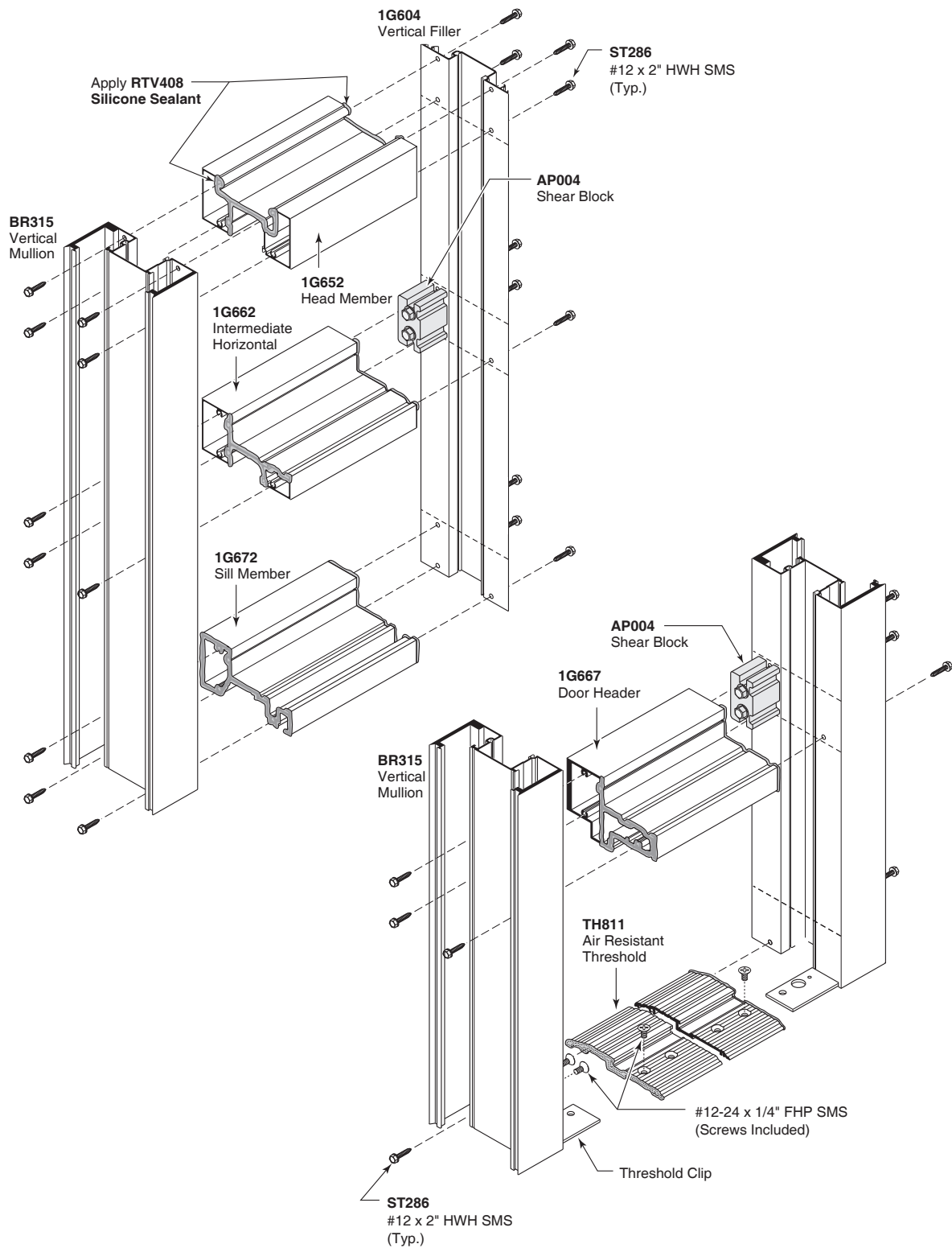
DETAIL K
