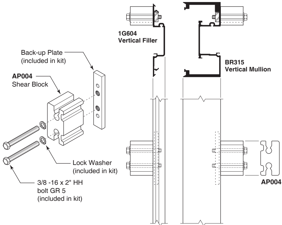
DETAIL J
