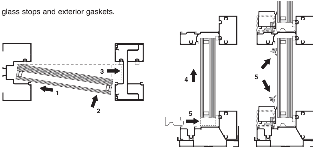
DETAIL FF
