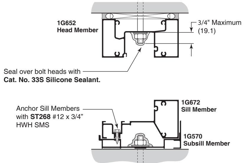
DETAIL BB
