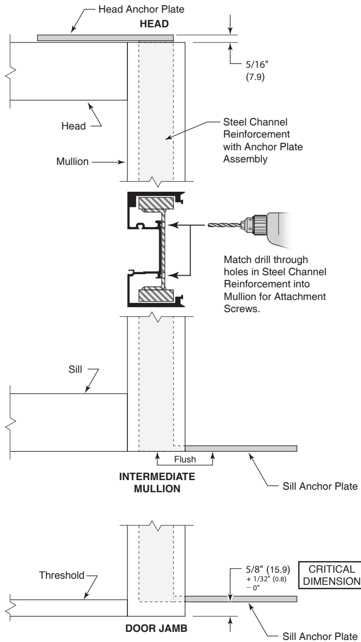
DETAIL N
