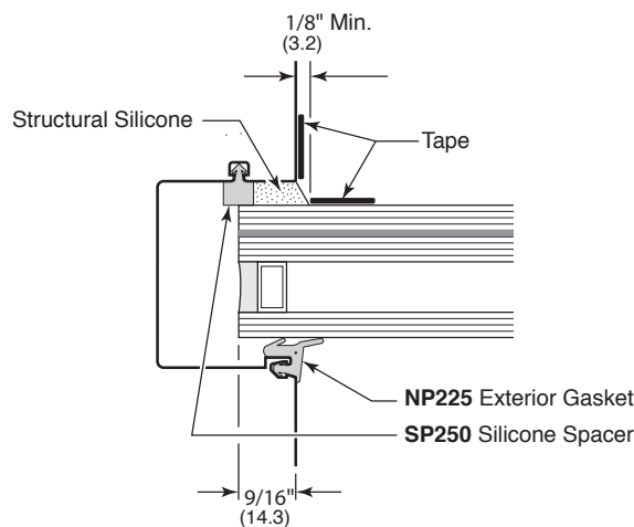
DETAIL GG
