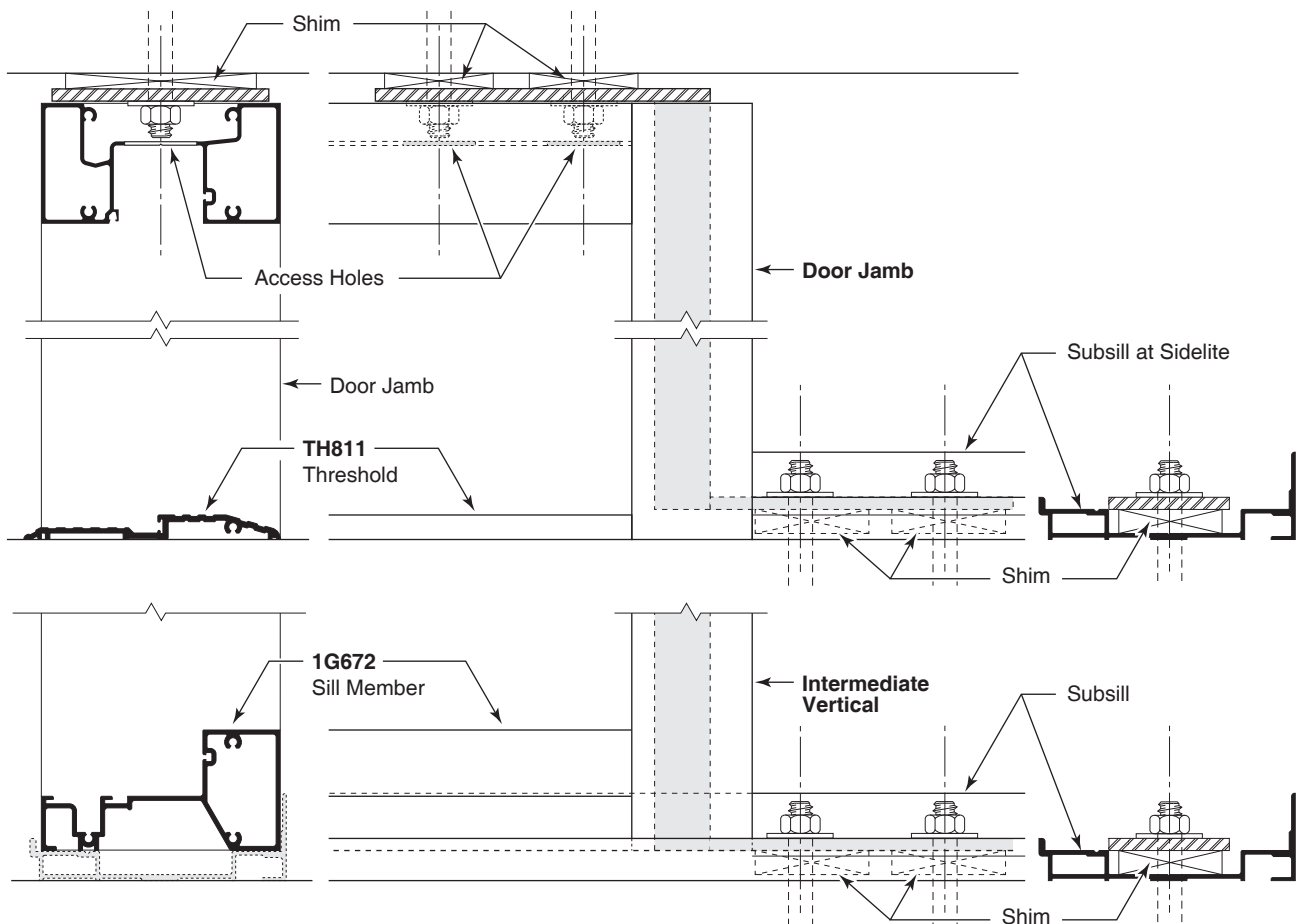
DETAIL W
