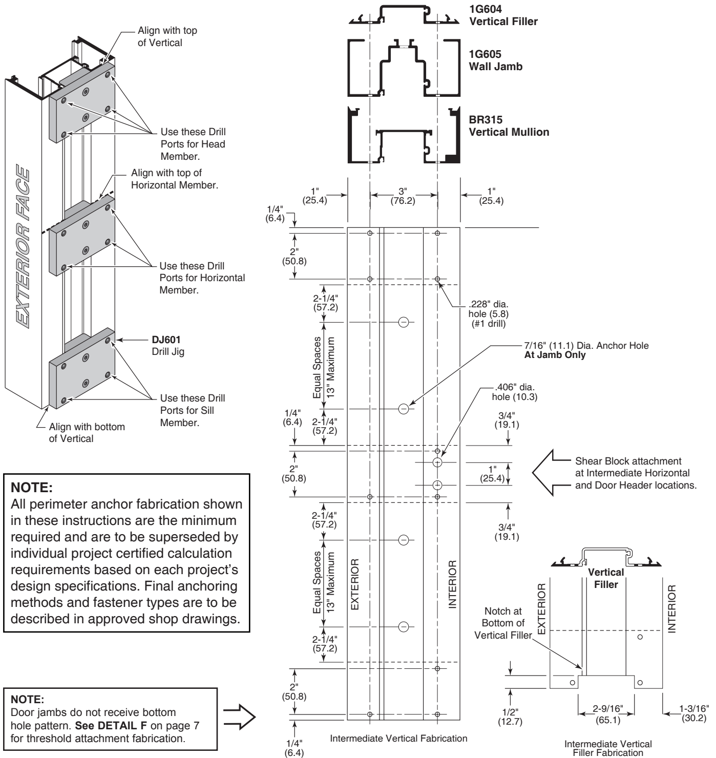
DETAIL E
