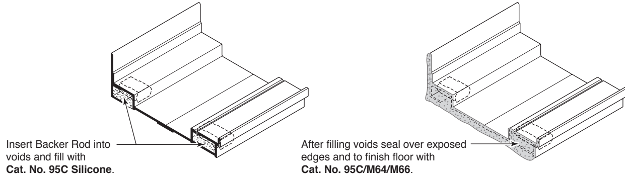
DETAIL V
